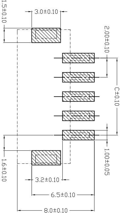
PCB Layout
